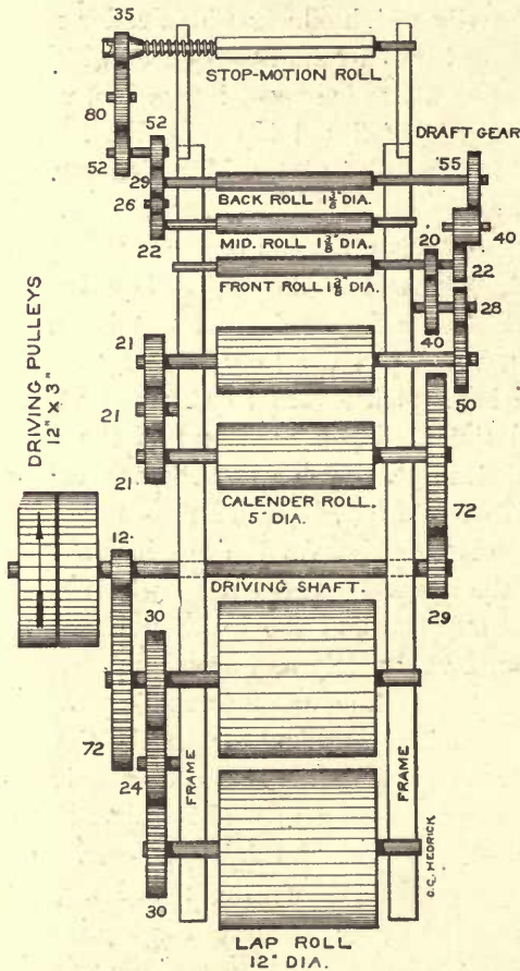
Fig. 100. Diagram of Gearing of Sliver Lap Machine.
